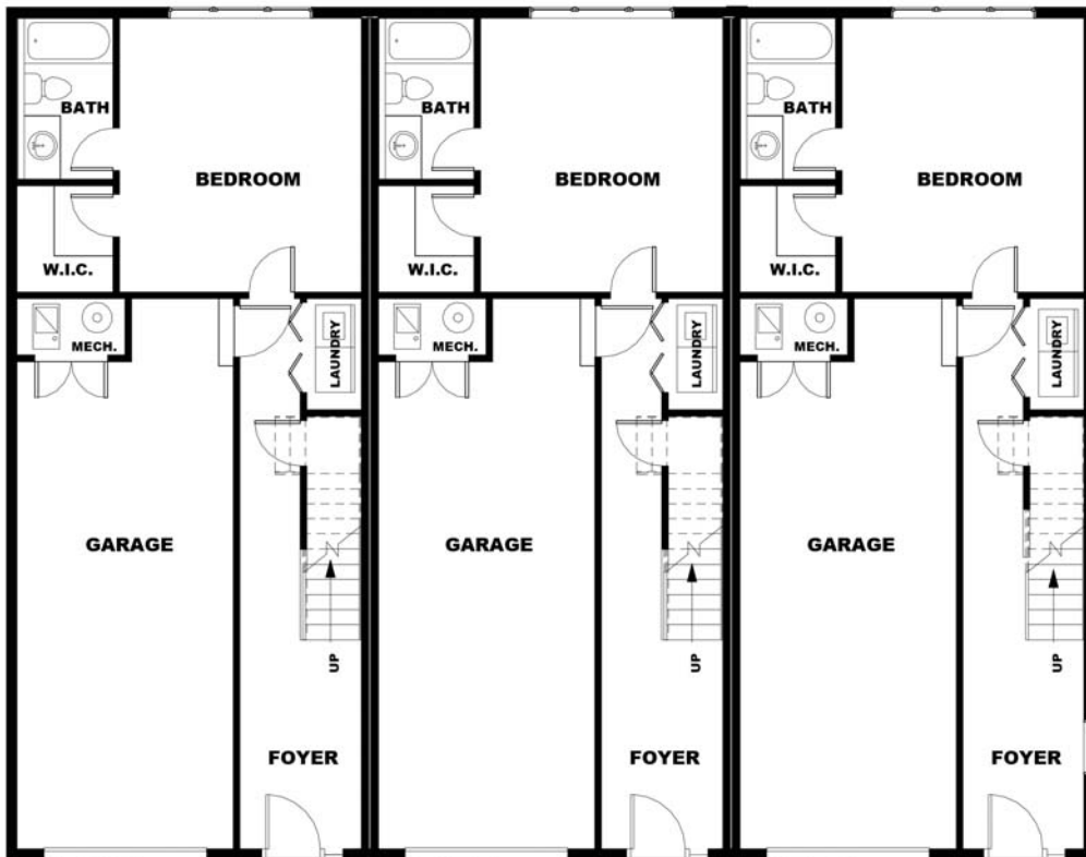
FIRST FLOOR 553 SQ. FT.
