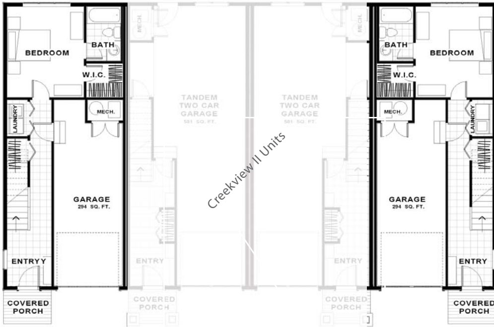
UNIT 1 FIRST FLOOR PLAN 458 SQ. FT.
